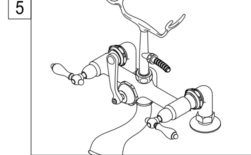
5. Place a washer between the side hole of the shower cradle and the cone nut of the shower hose. Tighten the cone nut.
